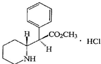
Figure 5: Structural Formula for Methylphenidate
