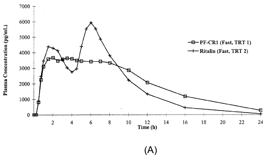
Figure 11. Study 97-147: mean methylphenidate time profiles under fast conditions (A) and fed conditions (B)
