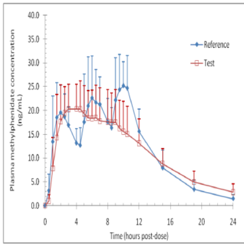
Figure 7: Mean (SD) Plasma Methylphenidate Concentration versus Time by Treatment after Single Dose under Fed Conditions (linear scale) - PK population Day 1 (A) and Day 12 (B)
