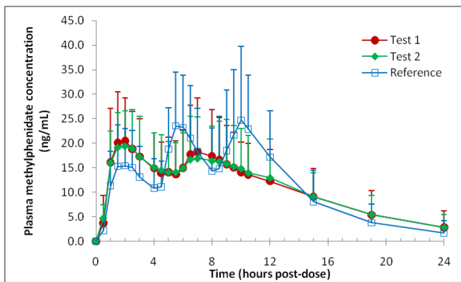
Figure 6: Plasma Concentrations for an 80 mg Dose of Aptensio in Adults Compared to 25 mg Ritalin IR Tid.
