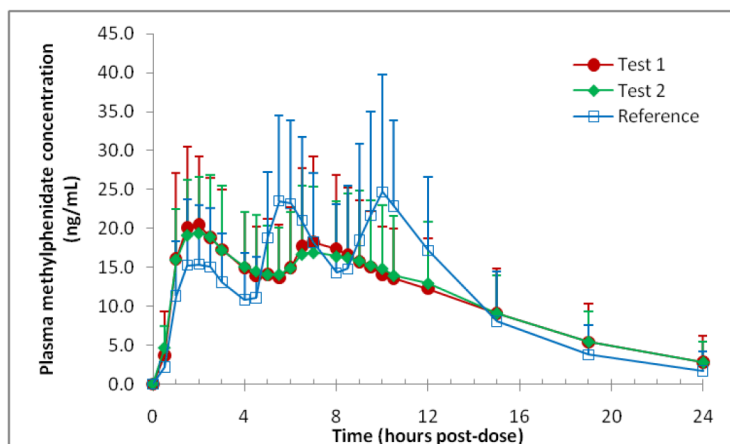
Figure 1: Mean (SD) plasma methylphenidate concentration versus time by treatment after single dose under fasted conditions (linear scale) - PK population
