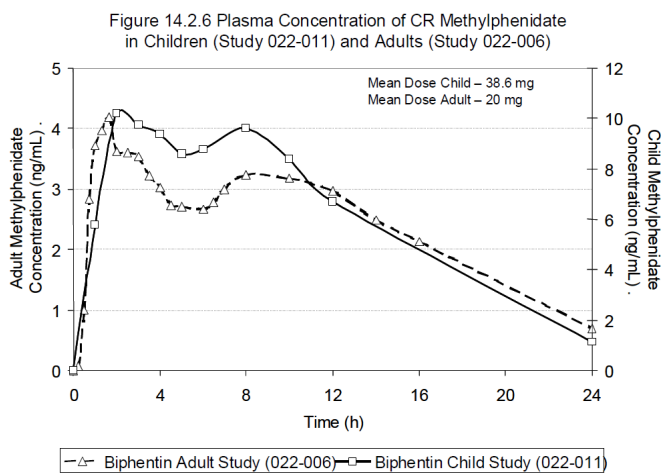
Figure 2: Mean Pharmacokinetic Profile of Methylphenidate for Children 6 Years and Above
