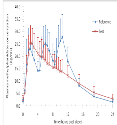
Figure 7: Mean (SD) Plasma Methylphenidate Concentration versus Time by Treatment after Single Dose under Fed Conditions (linear scale) - PK population Day 1 (A) and Day 12 (B)
